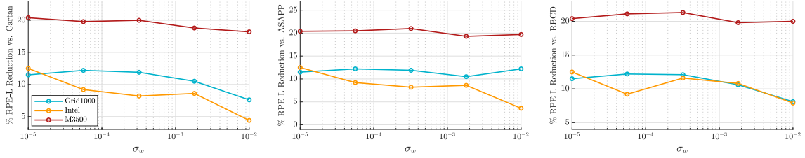
Fig. 2. Percentage reduction in RPE-L achieved by Algorithm 1 (ours) compared across the Grid1000, Intel, and M3500 datasets against centralized and distributed baselines with varying anisotropic noise levels \sigma_w : Cartan-Sync/SE-Sync (left), ASAPP (middle), and RBCD (right).
