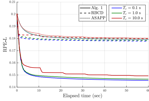
Fig. 4. The impact of varying the communication delay on RPE-L convergence over time for Algorithm 1, RBCD, and ASAPP. Each algorithm processed the M3500 dataset with \sigma_w = 10^{-2} for 60 seconds. We see that increased communication delays lead to slower convergence in general, but Algorithm 1 quickly achieves superior RPE-L in all cases.
